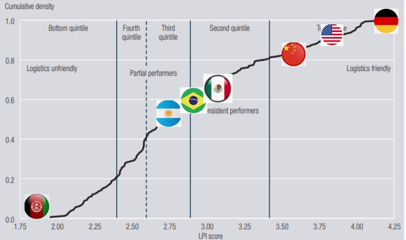
Figure 1.1 Cumulative distribution of LPI scores, 2018
